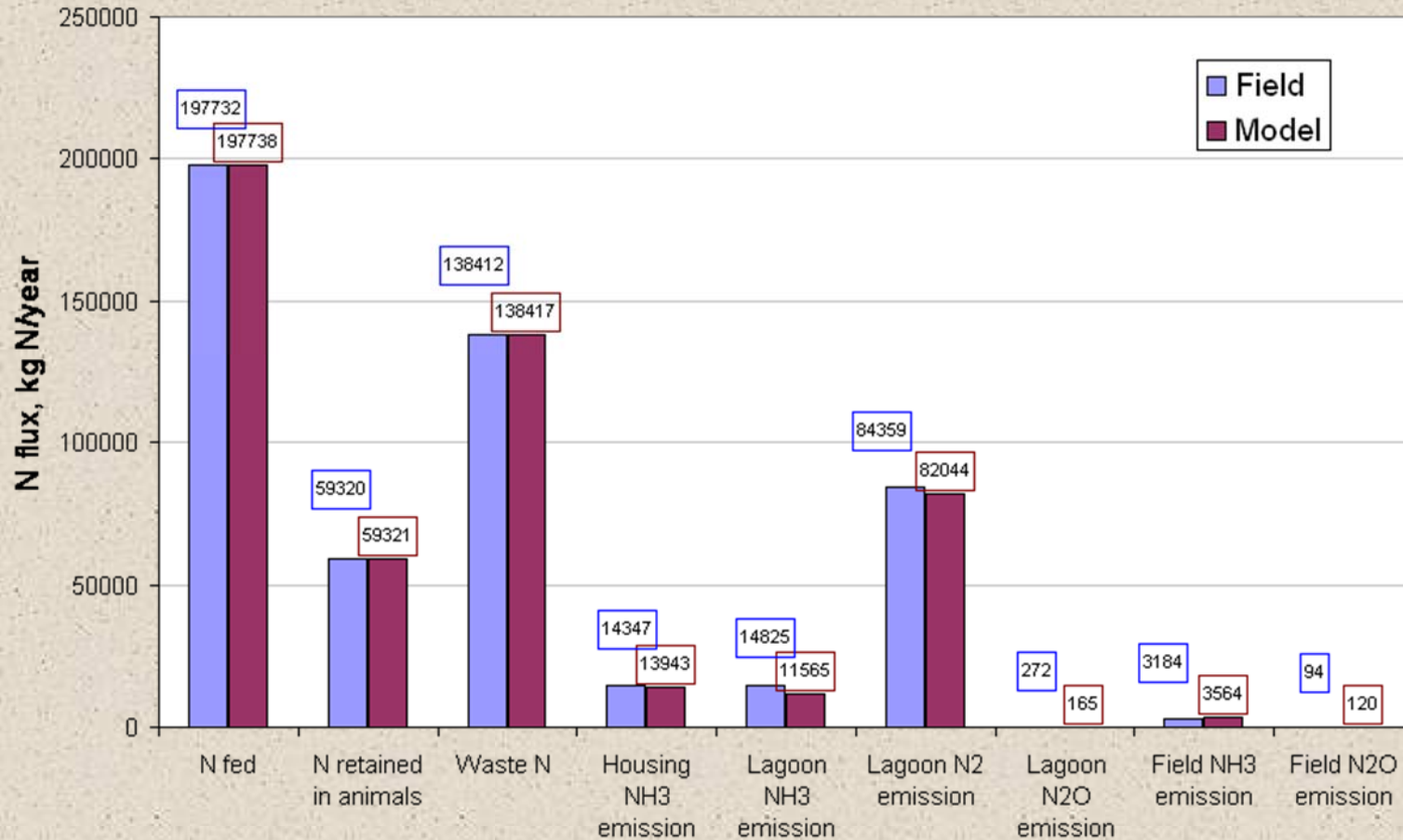
Measured and modeled N fluxes in a swine farm in the Coastal Plains of North Carolina in 1997-1998 (Field data from L.A. Harper et al., 2004)
